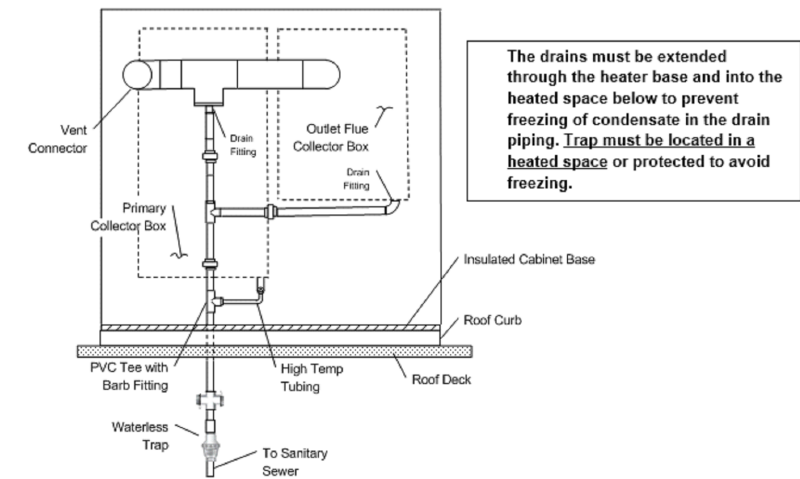
Figure 2 - Condensate Drain Piping
