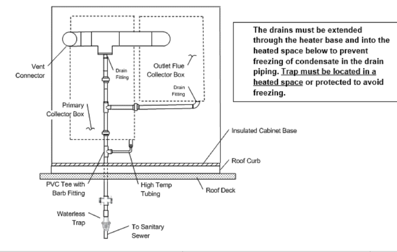
For outdoor installations run condensate drain from duct furnace into building (See Figure 2) Figure 2 - Condensate Drain Piping
