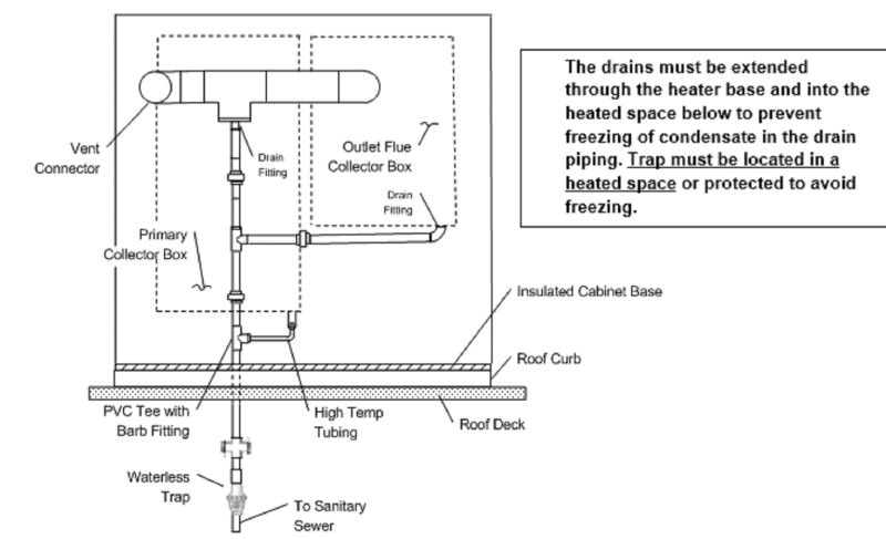
Figure 2 - Condensate Drain Piping
